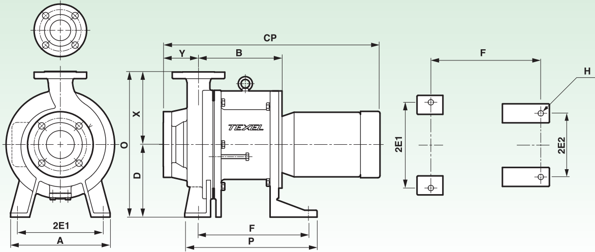
Model 0326, 4310, 6410
